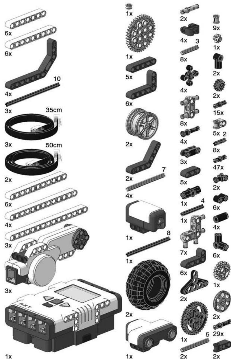
Figure 7-8. Mine Sweeper bill of materials
